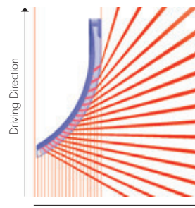
Angle of radiation by the wild animal reflector
